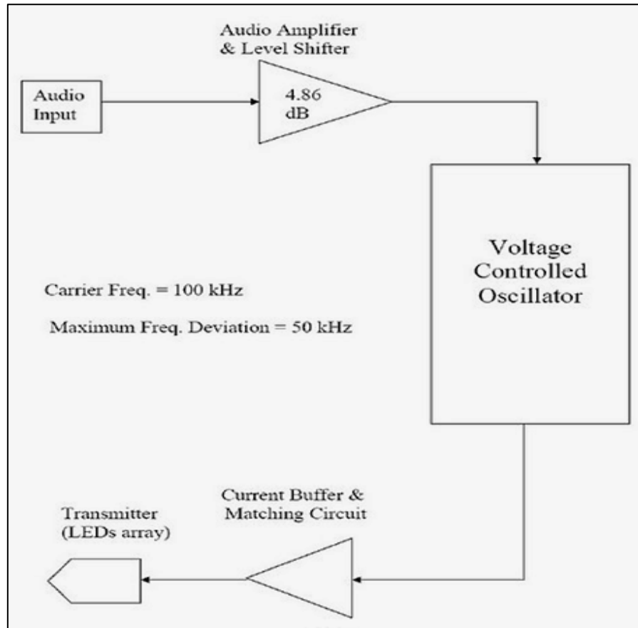
Figure- 2 Block diagram representing transmitter design.
