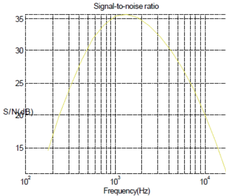
Figure-8: Measurement on the signal-to-noise ratio.
