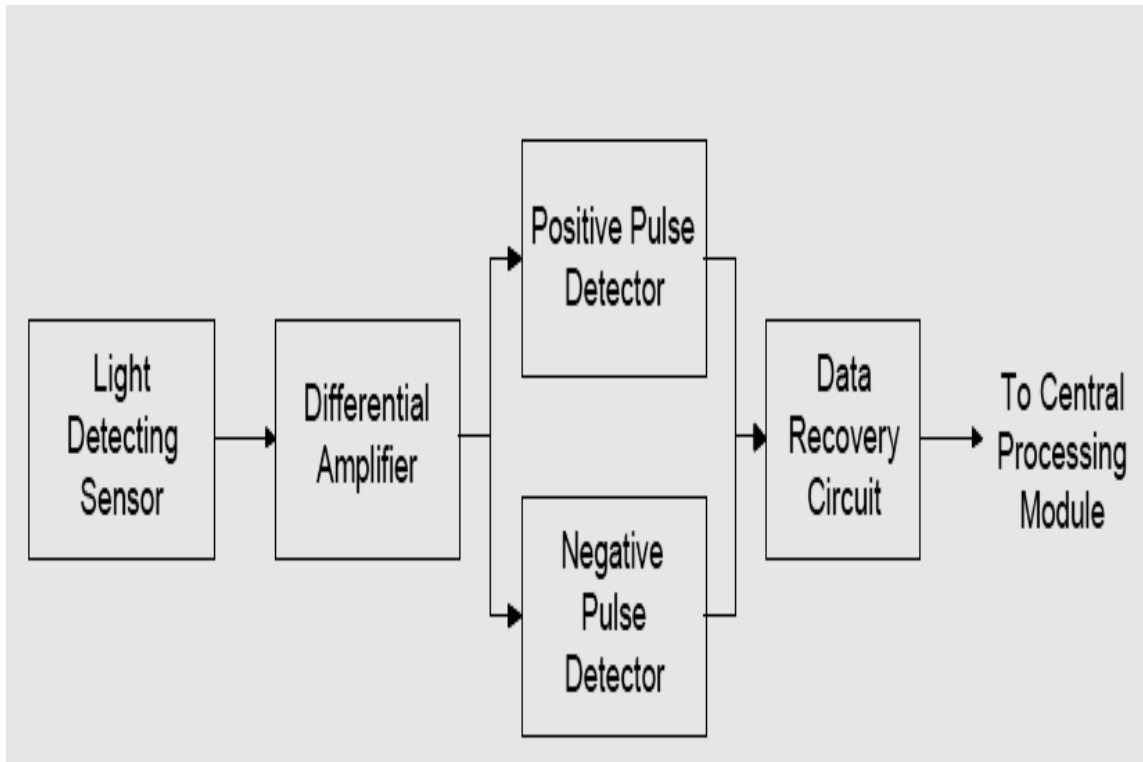
Figure-9: Visible light receiver
