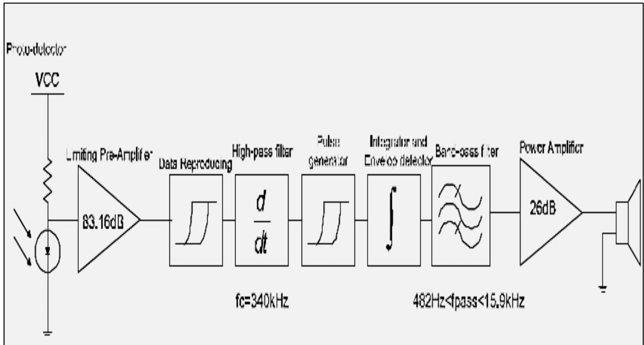
Figure- 3 Block diagram showing receiver design
