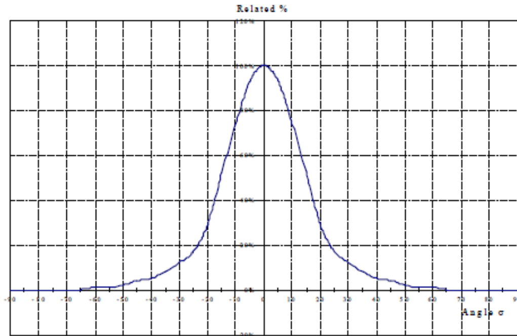
Figure-6: Radiation pattern of the LED traffic light.
